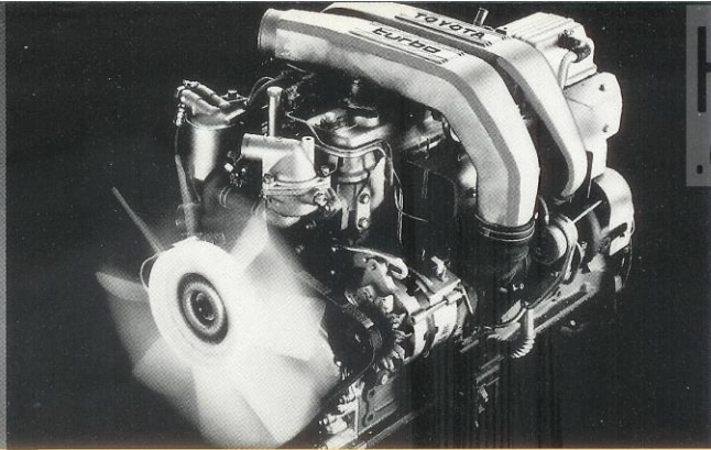
▲ 12H-T six cylinder turbo diesel. 100kW @ 3500 rpm. 315Nm @ 1800 rpm. Direct-injection turbo-charged diesel engine that delivers petrol-like performance with diesel economy.
