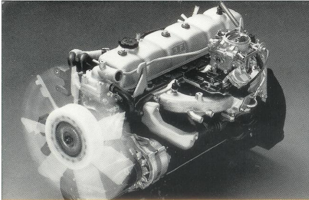
▲ 3F six cylinder petrol engine. 110kW @ 4200 rpm. 284Nm at 2200 rpm. Surpassing power without compromise.
